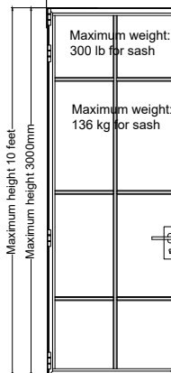
Maximum width - 5 feet for sash Maximum width - 1500 mm for sash
